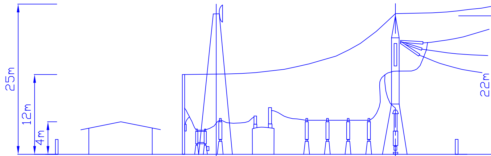
SECTION A
