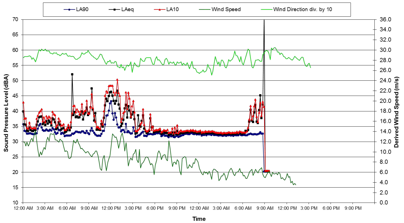
Location 10 Ambient Noise Data - 23 June 2011 and 24 June 2011
